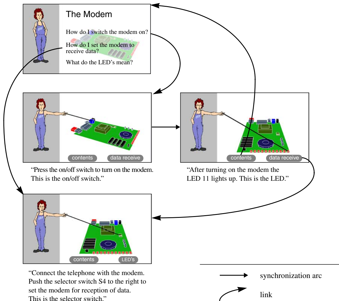
Figure 1. An example hypermedia presentation
