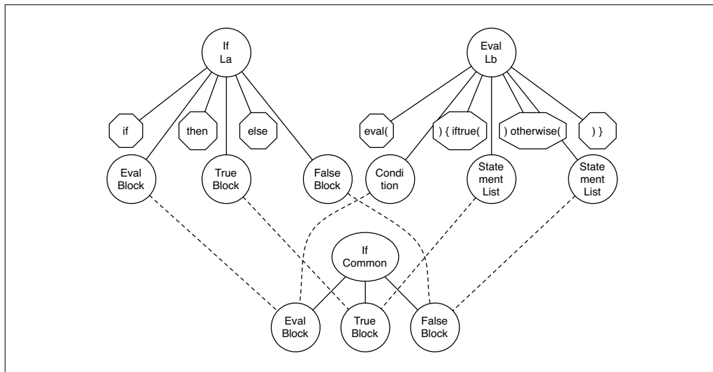
Fig. 5. Abstraction of a common construct.
