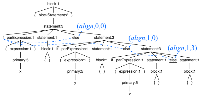
Figure 4. Alignment directives for nested if-else statements.
