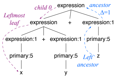
Figure 2. Parse tree for x+y+z; .
