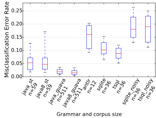
Figure 5. Standard box-plot of leave-one-out validation error rate between formatted document d' and original d .
