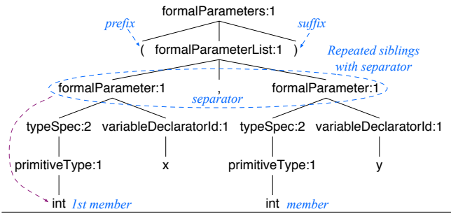
Figure 3. Formal Args Parse Tree void f(int x, int y).
