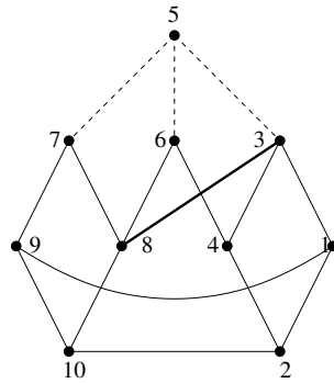
Fig. 5. A drawing of C_5 \times C_2 with 3 as the root node.
