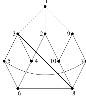
Fig. 3. A drawing of C_5 \times C_2 with 1 as the root node.
