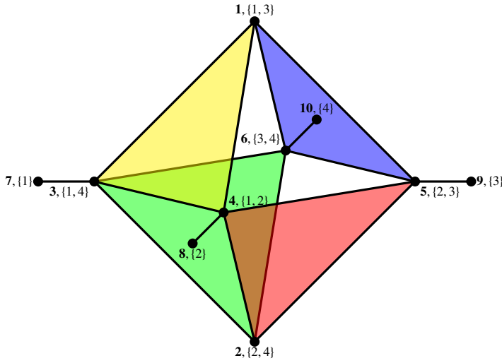
Fig. 2 Three-dimensional illustration of the coordination game used to show that 3-equilibria do not exist (Theorem 5). The colored facets indicate the triangles that can be unicolored. The identity of the players is displayed in boldface. The strategy sets of the players are stated between curly braces.
