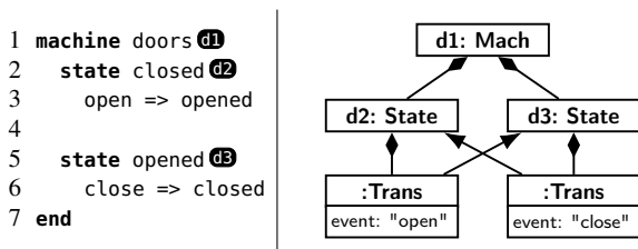
Fig. 3: Doors 1 : a simple textual representation of a state machine and its model.
