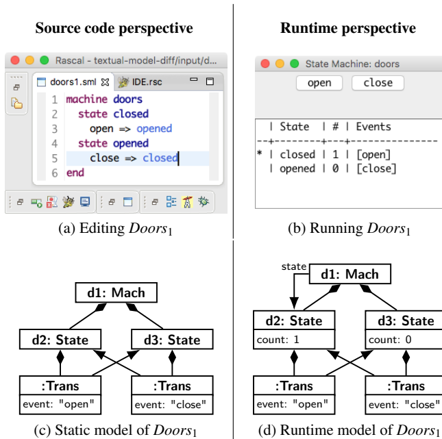
Fig. 13: LiveSML: the left shows the source code perspective with the IDE at the top and the static model at the bottom. The right shows the runtime perspective with the state machine GUI at the top, and the (extended) run-time model at the bottom.
