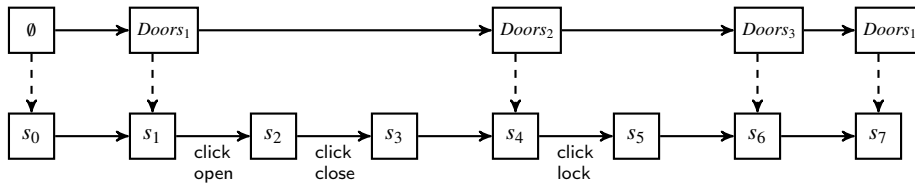
Fig. 15: Interleaved coevolution of models Doors_n and application run-time states s_n over time
