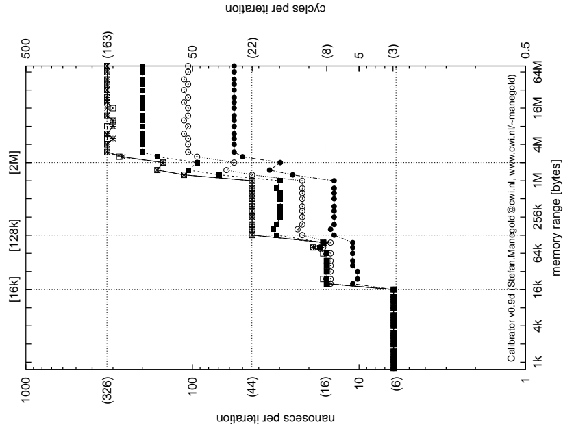
ia-64.cache-replace-time
