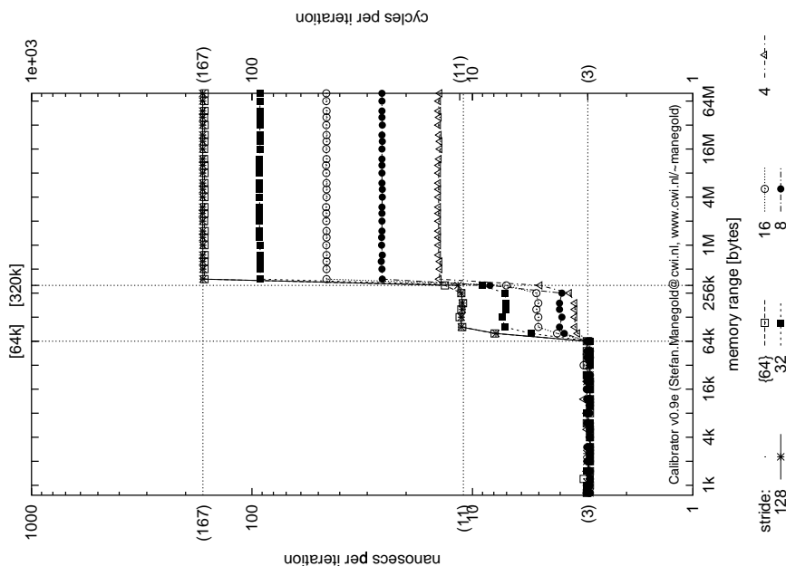
Thunderbird-1000.cache-miss-latency
