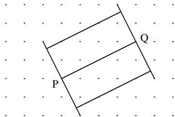
Fig. 1. Smallest triangle based on pebbles P, Q .
