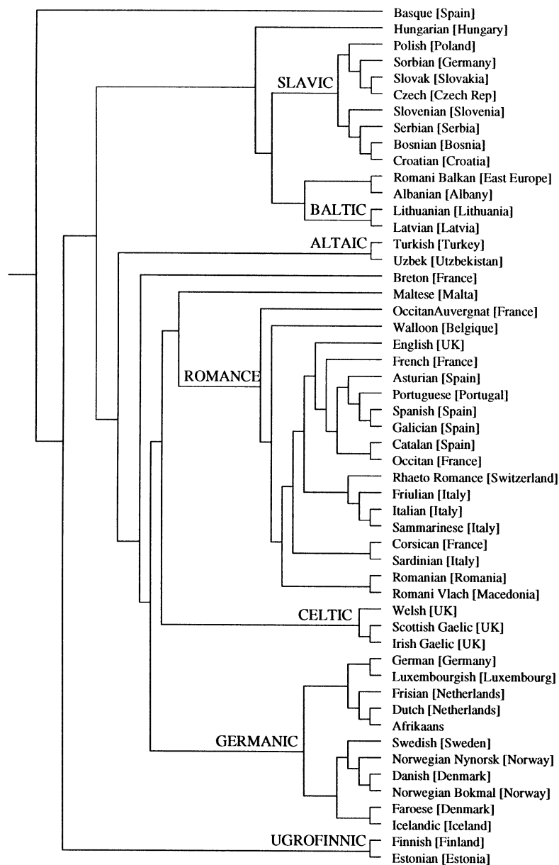
Fig. 5. The language tree using approximated normalized information distance, d -version (V.3), and the Fitch–Margoliash method.
