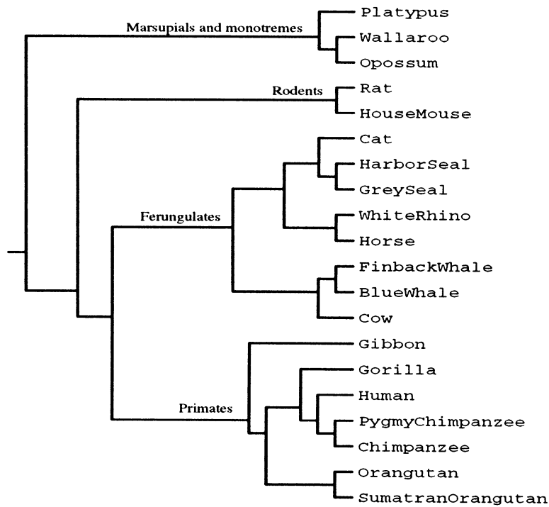
Fig. 3. The evolutionary tree built from complete mammalian mtDNA sequences using the similarity metric.
