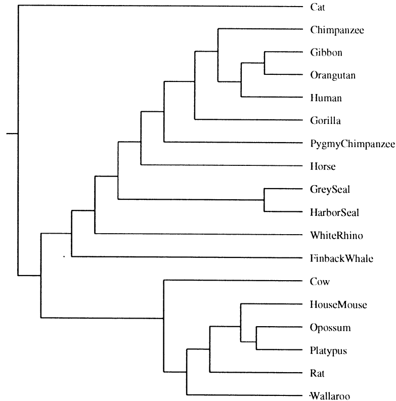
Fig. 1. The evolutionary tree built from complete mammalian mtDNA sequences using frequency of k -mers.
