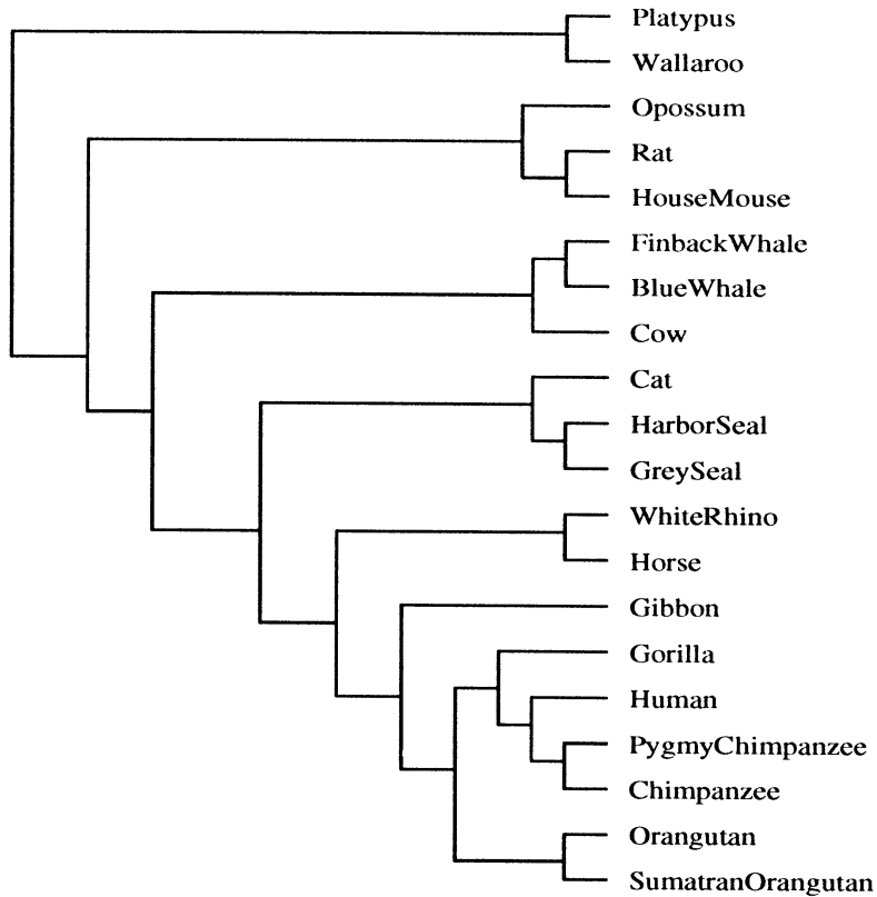
Fig. 2. The evolutionary tree built from complete mammalian mtDNA sequences using block size k = 7 and d' .
