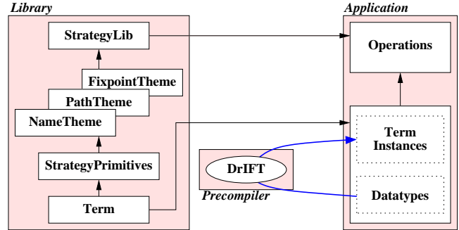
Figure 4. Strafunski = Library + Precompiler
