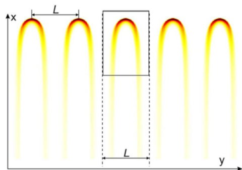
FIGURE 6. An array of streamers as simulated with a periodic boundary condition. It is found that the streamer separation is equal to the streamer diameter and that the electric field inside the streamer goes to zero due to screening. Figure taken from ref. [22].
