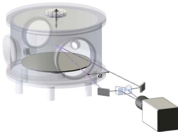
FIGURE 2. A stainless steel vessel of 50 cm diameter and 30 cm height is used to create a 16 cm gap in a controlled gas composition. The large side window offers the possibility to view the streamer under two angles. Details on the set-up and its pulsed power supply can be found elsewhere 1,14 .
