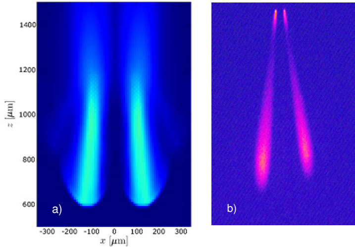
FIGURE 4a). Two negative streamers in nitrogen at atmospheric pressure advancing downwards and repelling each other; shown are surfaces of constant electron density in an advanced state of evolution within a constant background field.
