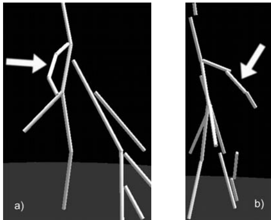
FIGURE 3a). The front view of a streamer that appears to reconnect as in circle 2 of fig. 1a.
