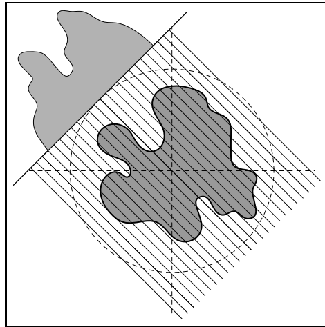
Fig. 14. A planar black-and-white image with one of its projections. If strip projections are used, the total amount of “black” in a set of consecutive strips parallel to the projection direction is measured.
