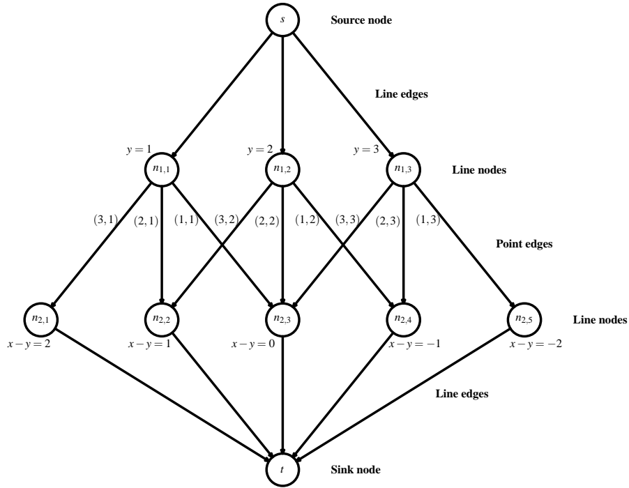
Fig. 2. Associated graph G for the triple (A, v^{(1)}, v^{(2)}) from Fig. 1.
