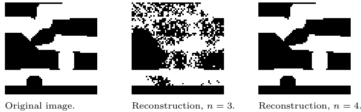
Fig. 9. (a) Original image; (b) Reconstruction from three projections (horizontal, vertical, diagonal) that has exactly the prescribed projections; (c) Perfect reconstruction of the original image from four projections (horizontal, vertical, diagonal, anti-diagonal).
