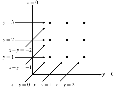
Fig. 1. Example lattice: A = \{1, 2, 3\} \times \{1, 2, 3\} , v^{(1)} = (1, 0) , v^{(2)} = (1, 1) .
