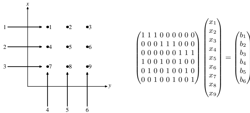
Fig. 7. (a) (left) Numbering scheme for the lattice points and the lattice lines in a rectangular reconstruction lattice; (b) (right) System of equations corresponding to the numbering in (a).
