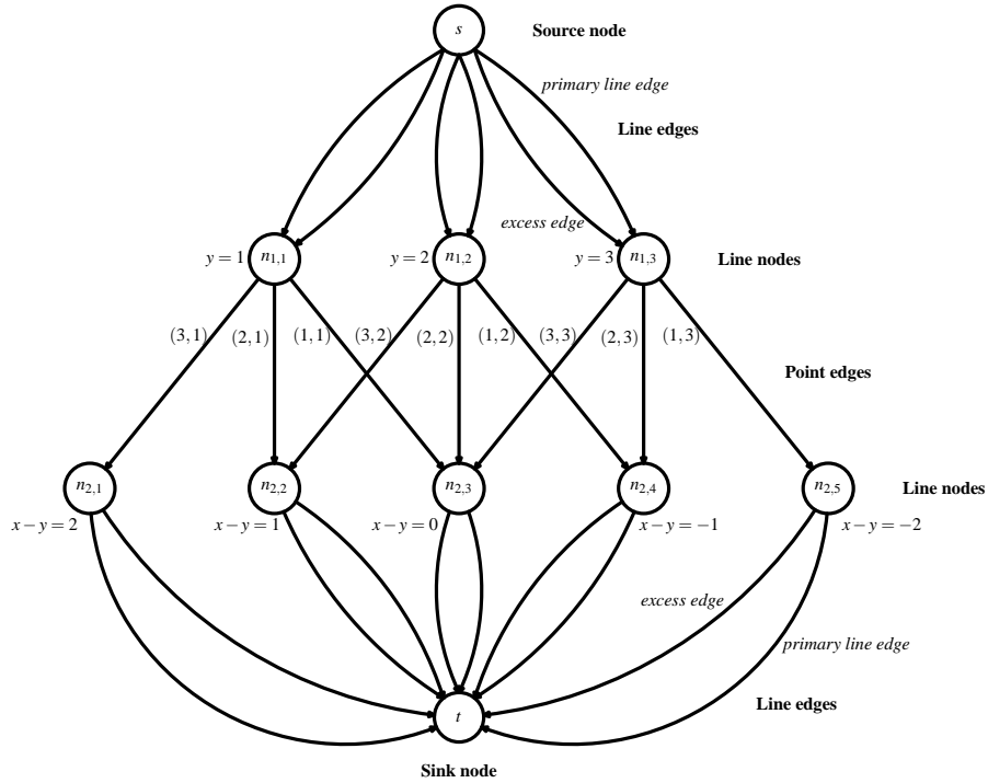
Fig. 5. Modified associated graph G' for the triple (A, v^{(1)}, v^{(2)}) from Fig. 1.
