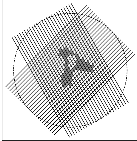
Fig. 15. Two parallel beams span a pixel grid. On this pixel grid, network flow methods can be used to solve the two-projection 0-1 reconstruction problem.
