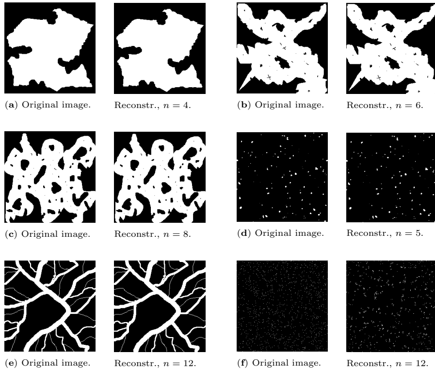
Fig. 8. Six original images and their reconstructions. The number n of projections is shown in the figure caption.
