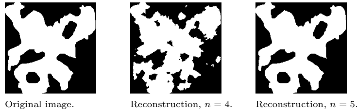
Fig. 10. (a) Original image; (b) Reconstruction from four projections, which does not have the prescribed projections. The horizontal and vertical projections are identical to those of the first image. The diagonal and anti-diagonal projections have a total projection difference (sum of absolute values) of 184 and 126 respectively. (c) Perfect reconstruction of the original image from five projections.
