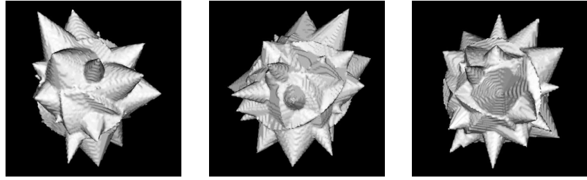
(a) Cones pointing out, 128 \times 128 \times 128 : perfect reconstruction from 4 projections.
