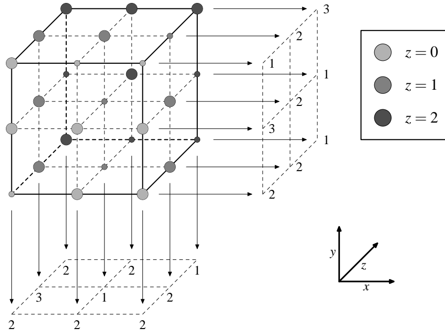
Fig. 11. 3 \times 3 \times 3 binary volume with its projections in directions v^{(1)} = (1, 0, 0) and v^{(2)} = (0, 1, 0) . A large circle indicates a value of 1; a small circle indicates a value of 0.
