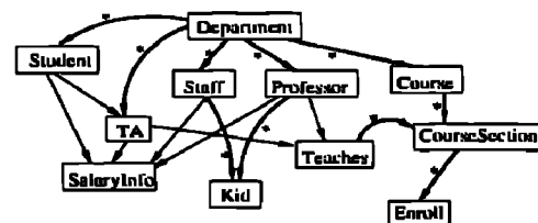
Figure 4.1 DTD graph of Department dataset
