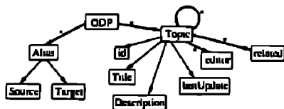
Figure 4.2 DTD graph of the ODP dataset
