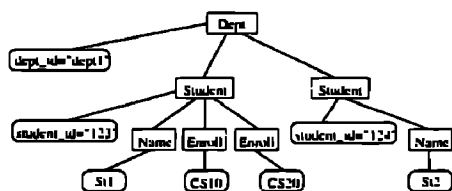
Figure 3.2 The graph representation of "Dept.xml"
