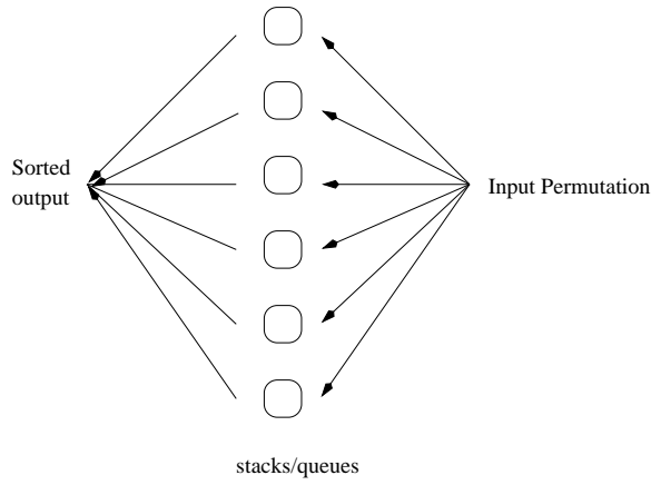
Figure 2: Six stacks/queues arranged in parallel order
