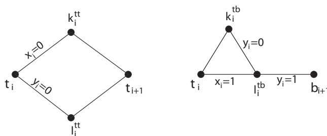
■ Figure 2 Two gadgets used to modify the reduction from Parity in the query complexity model to one for Inner Product in communication complexity. On the left the gadget replacing the top z_i = 0 edge in Fig 1; on the right the gadget for the diagonal top-to-bottom z_i = 1 edge.
