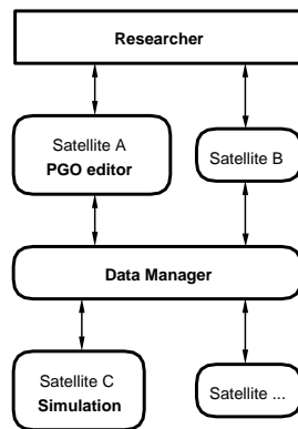
Fig. 1. Architecture of the Computational Steering Environment.
