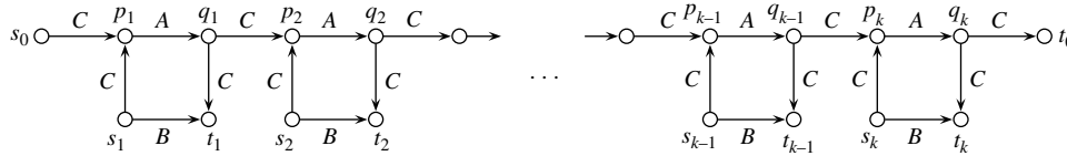
FIGURE 1. The graph G_k used in the proof of Theorem 3.1. Arcs are labeled with their types.
