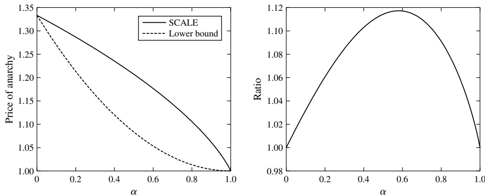
FIGURE 5. Lower bound for arbitrary Stackelberg strategies vs. upper bound of SCALE for linear latency functions (left) and the respective ratio (right).
