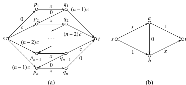
FIGURE 6. (a) Generalized Braess instance used in the proof of Theorem 6.3. (b) Braess instance. Arcs are labeled with their latency functions.
