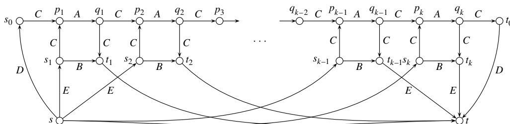
FIGURE 3. The graph G_k used in the proof of Theorem 3.2. Arcs are labeled with their types.
